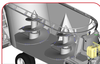
Double auger for a homogeneous mix
